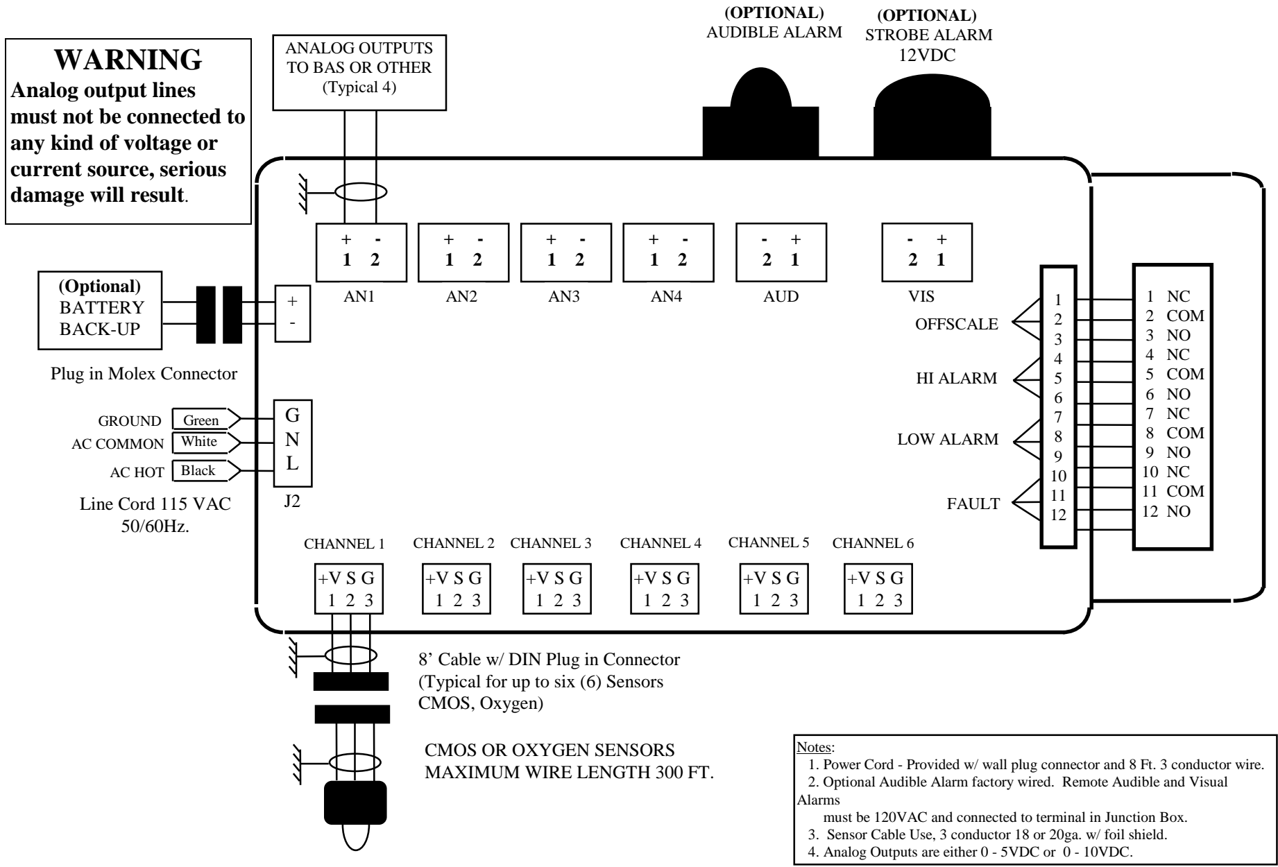
Figure 10 - Wiring Diagram
